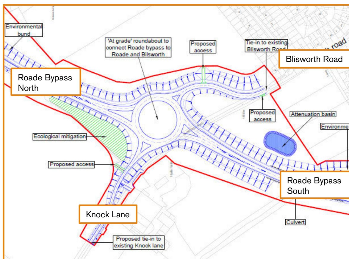
Figure 4: Blisworth Road/Knock Lane/Roade bypass 4-arm roundabout
