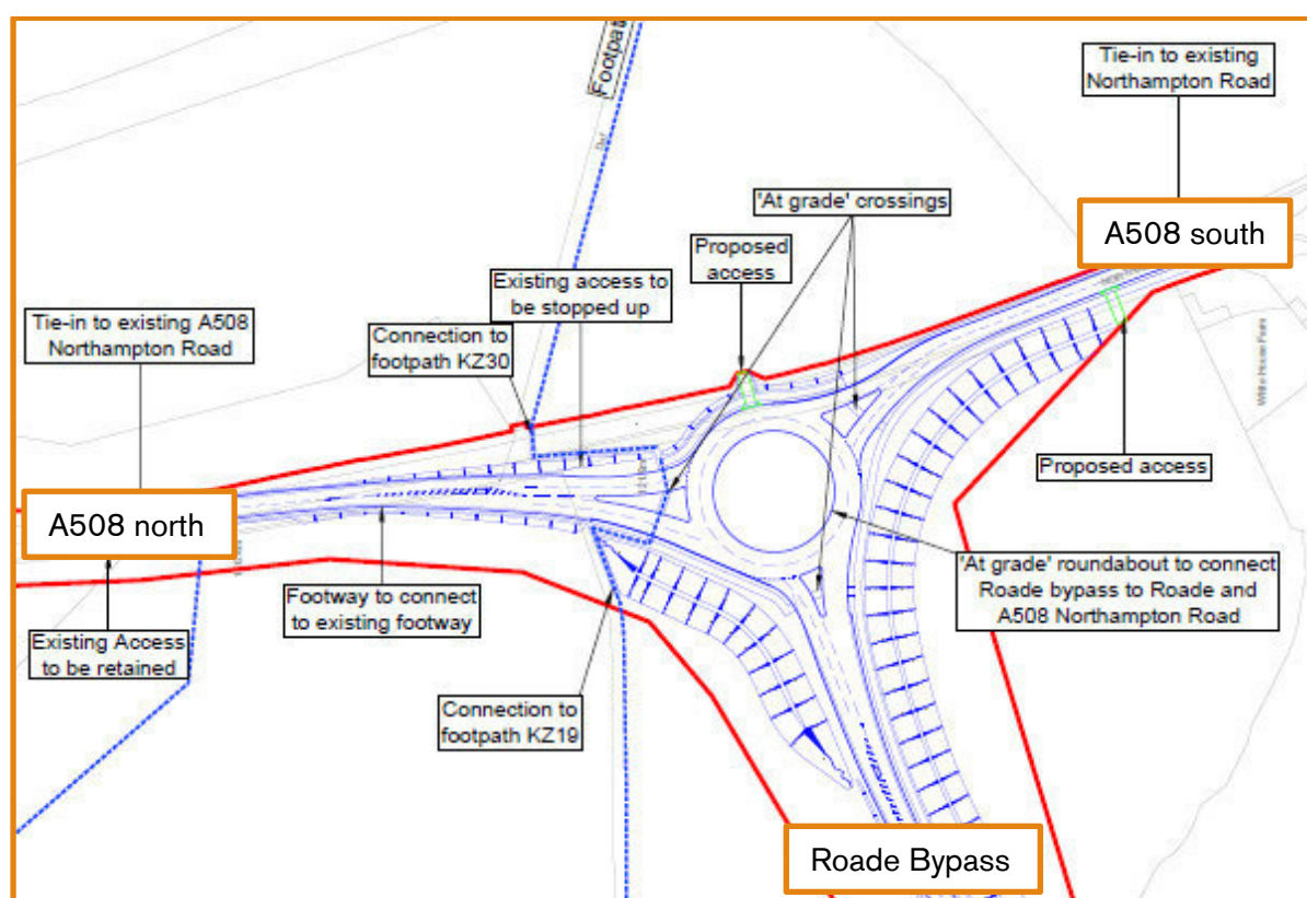
Figure 5: A508 Northampton Road/Road Bypass 3-arm roundabout
