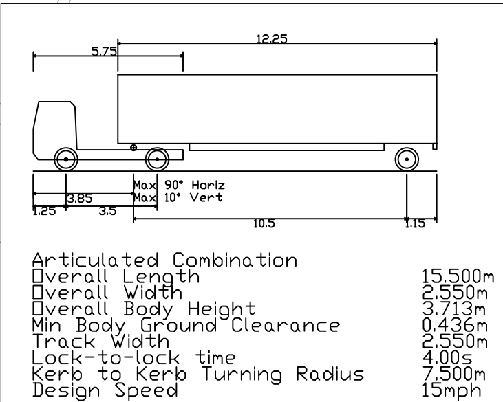
15.5m Long Articulated Combination
